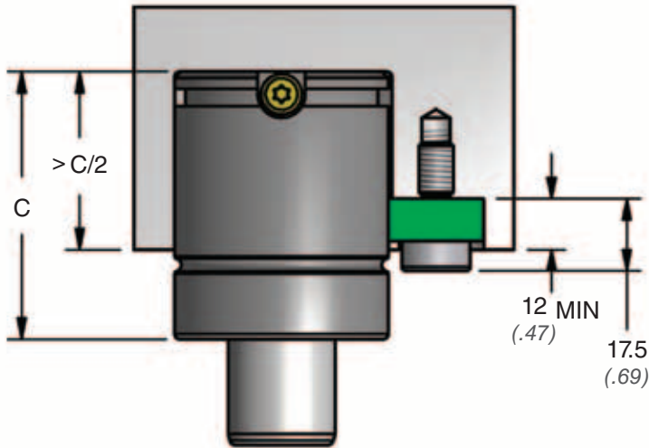
For "C" Dimension, refer to appropriate DADCO product catalog.
