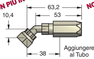
90.504.654 (S-654) Raccordo Tubo a 45° (per Y-250)
