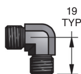
90.508.201 (D-201) Raccordo a L
