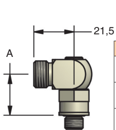
90.506.230 (S-230) Raccordo a 90°
