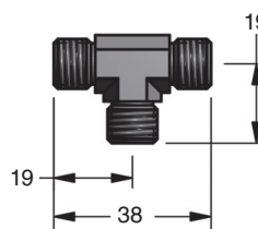
90.508.401 (D-401) Raccordo a T
