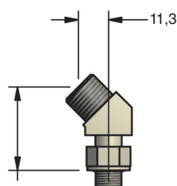
90.505.330 (S-330) Raccordo a 45°
