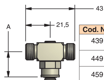
90.506.439 (S-439) Raccordo a T
