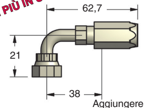
90.504.659 (S-659) Raccordo Tubo a 90° (per Y-250)
