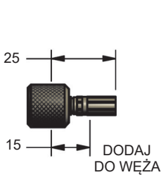
90.804.943 Prosty Adapter Portu (B-943)
